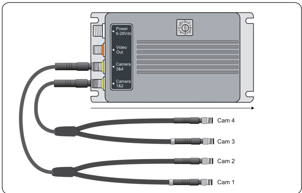
micro-FourSight-C System Diagram
