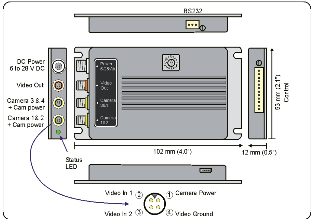
micro-FourSight-C System Diagram
