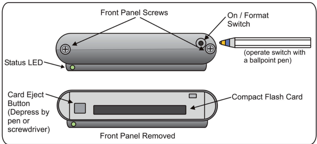
FlashBack-2 On/Format Button and Removing / Replacing the Internal CF Card
